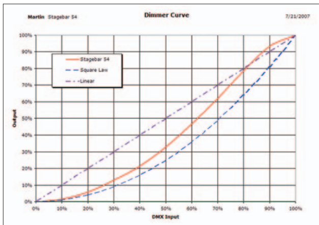
Fig 7: Dimmer Curve.
