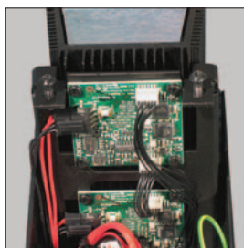
Fig 10: LED Electronics.
